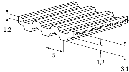
AT5-DL Tooth Form
