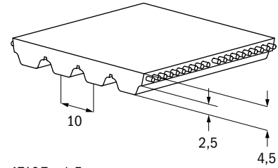
AT10 Tooth Form
