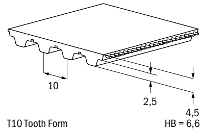
T10 Tooth Form
