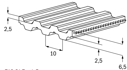
T10-DL Tooth Form
